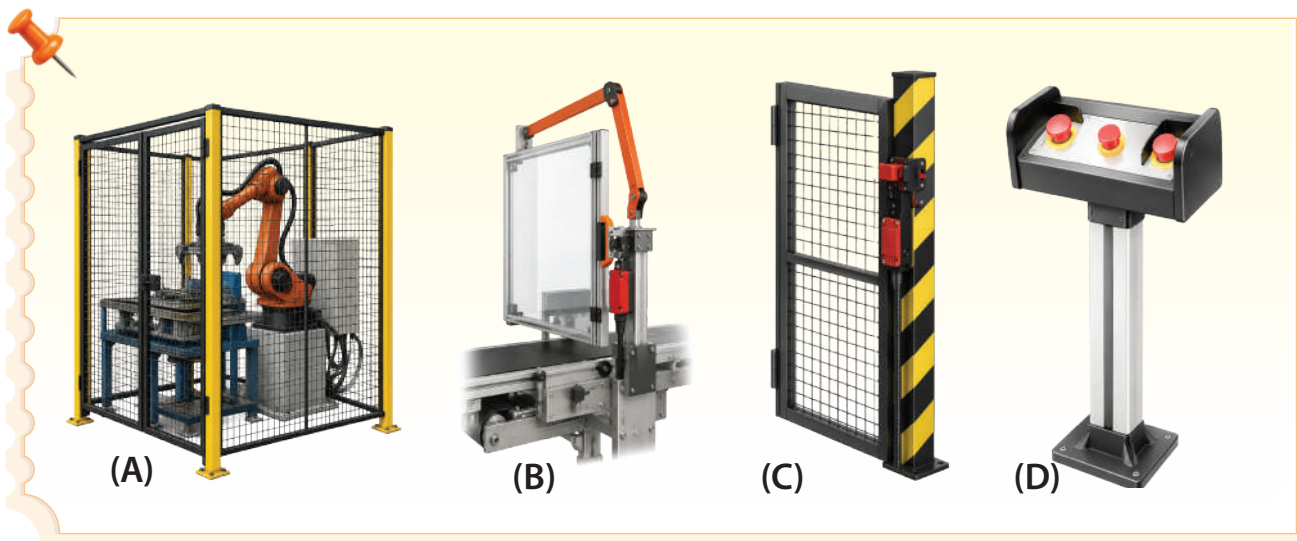
Examples of work-equipment engineering controls: (a) fixed guard, (b) adjustable guard with interlock, (c) interlocked guard and (d) two-hand control device. These measures help prevent or control access to hazardous machine functions and danger zones.
